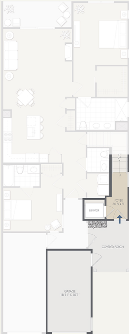
ENTRY/GARAGE LEVEL
